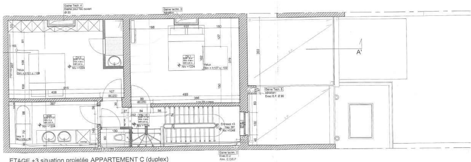
ETAGE +3 situation projetée APPARTEMENT C (duplex) Surface brut: Etage 2 = 77.31 m 2 Etage 3 = 66.7 m 2 Total = 144.01 m 2
